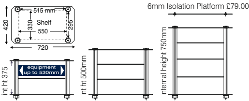
TV Support (hwd 440 x 720 x 420) Sound Support (hwd 565 x 720 x 420) Sound Tower (hwd 815 x 720 x 420)
