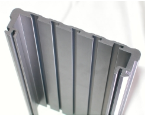
Custom Stands Unique extrusion designed for maximum heat dissipation and mechanical contact and neatly housing HDD.
